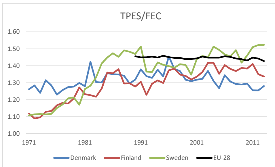
Figure 7. Trend of energy efficiency of the energy transformation system in Denmark, Finland and Sweden, 1971-2013. Total primary energy supply (TPES in Mtoe) divided by final energy consumption (FEC in Mtoe). The lower the ratio, the better the efficiency. Data source: IEA 2015.
