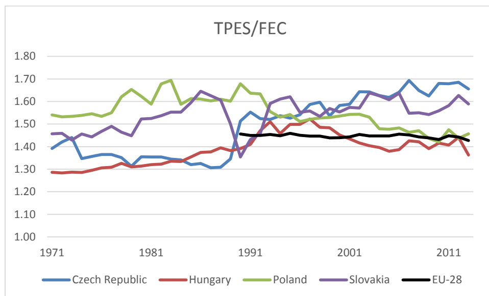
Figure 10. Trend of energy efficiency of the energy transformation system in Czech Republic, Hungary, Poland and Slovakia, 1971-2013. Total primary energy supply (TPES in Mtoe) divided by final energy consumption (FEC in Mtoe). The lower the ratio, the better the efficiency. Data source: IEA 2015.
