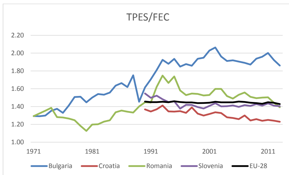
Figure 11. Trend of energy efficiency of the energy transformation system in Bulgaria, Croatia, Romania and Slovenia, 1971/1990-2013. Total primary energy supply (TPES in Mtoe) divided by final energy consumption (FEC in Mtoe). The lower the ratio, the better the efficiency. Data source: IEA 2015.
