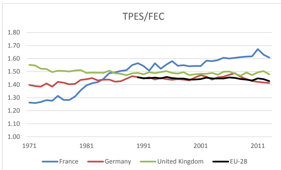
Figure 6. Trend of energy efficiency of the energy transformation system in France, Germany and the United Kingdom, 1971-2013. Total primary energy supply (TPES in Mtoe) divided by final energy consumption (FEC in Mtoe). The lower the ratio, the better the efficiency. Data source: IEA 2015.
