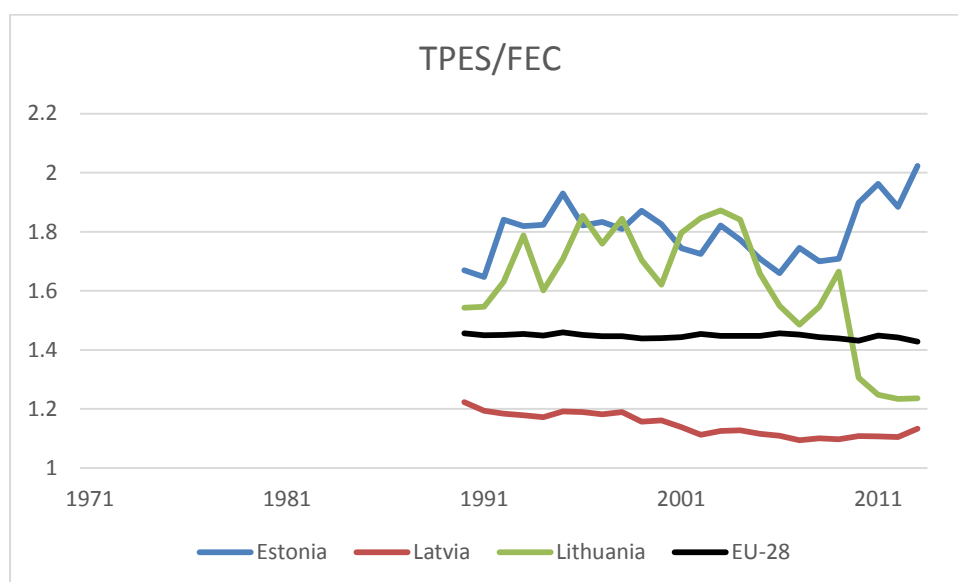
Figure 9. Trend of energy efficiency of the energy transformation system in Estonia, Latvia and Lithuania, 1990-2013. Total primary energy supply (TPES in Mtoe) divided by final energy consumption (FEC in Mtoe). The lower the ratio, the better the efficiency. Data source: IEA 2015.
