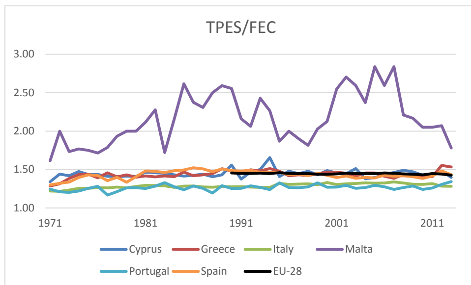
Figure 5. Trend of energy efficiency of the energy transformation system in Cyprus, Greece, Italy, Malta, Portugal and Spain, 1971-2013. Total primary energy supply (TPES in Mtoe) divided by final energy consumption (FEC in Mtoe). The lower the ratio, the better the efficiency. Data source: IEA 2015.
