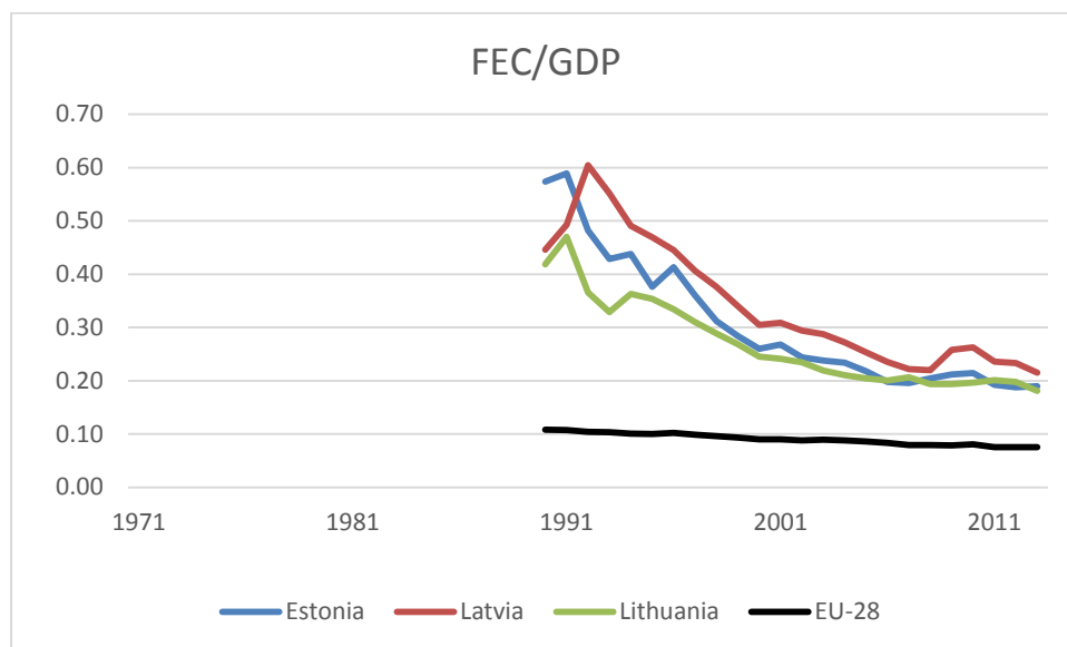
Figure 16. Trend of energy intensity in Estonia, Latvia and Lithuania, 1990-2013. Final energy consumption (FEC) divided by gross domestic product (GDP), Mtoe/1000 USD 2005 . Data source: IEA 2015.
