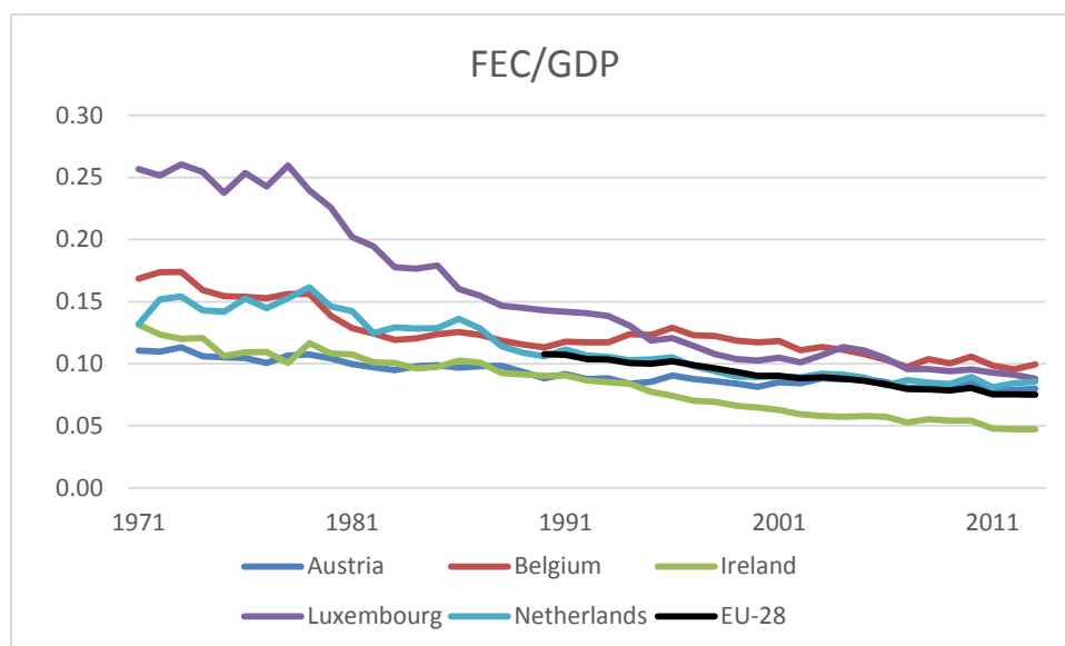
Figure 15. Trend of energy intensity in Austria, Belgium, Ireland, Luxembourg and the Netherlands, 1971-2013. Final energy consumption (FEC) divided by gross domestic product (GDP), Mtoe/1000 USD 2005 . Data source: IEA 2015.
