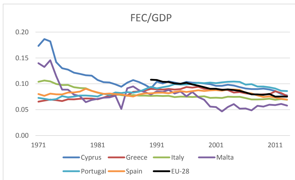
Figure 12. Trend of energy intensity in Cyprus, Greece, Italy, Malta, Portugal and Spain, 1971-2013. Final energy consumption (FEC) divided by gross domestic product (GDP), Mtoe/1000 USD 2005 . Data source: IEA 2015.
