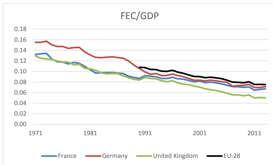
Figure 13. Trend of energy intensity in France, Germany, and the United Kingdom, 1971-2013. Final energy consumption (FEC) divided by gross domestic product (GDP), Mtoe/1000 USD 2005 . Data source: IEA 2015.
