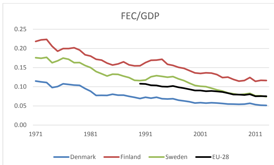
Figure 14. Trend of energy intensity in Denmark, Finland and Sweden, 1971-2013. Final energy consumption (FEC) divided by gross domestic product (GDP), Mtoe/1000 USD 2005 . Data source: IEA 2015.
