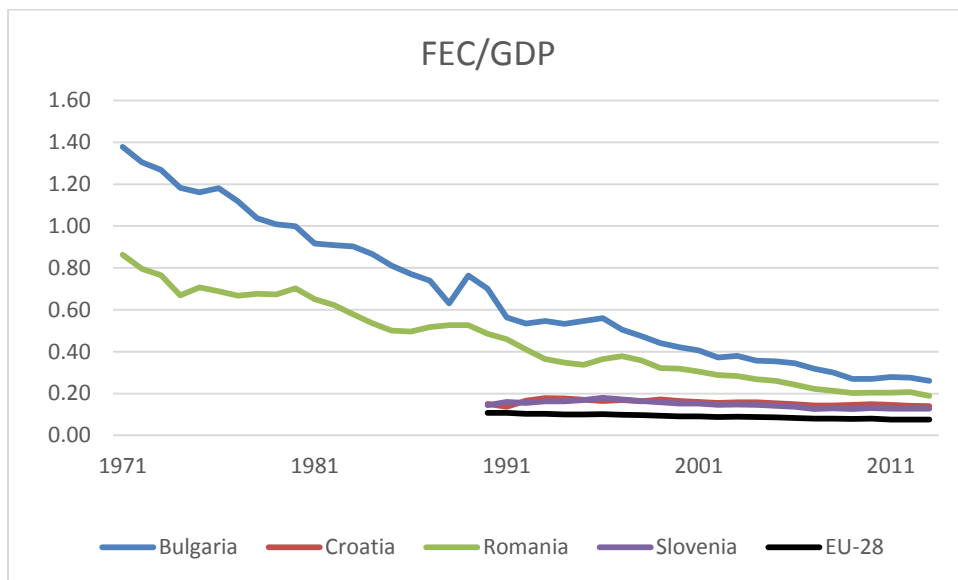
Figure 18. Trend of inverse energy efficiency (energy intensity) of the national economy in Bulgaria, Croatia, Romania and Slovenia, 1971/1990-2013. Final energy consumption (FEC) divided by gross domestic product (GDP), Mtoe/1000 USD 2005 . Data source: IEA 2015.
